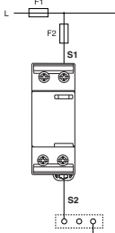
TN-S system, T-connection
