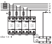
IT system, V-connection (only products with Uc 440V, only if F1 ≤ 100A)
